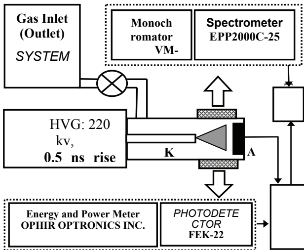
Fig. 1. Experimental setup: 1 – discharge chamber, 2 – CaF 2 window, K – cathode, A – anode
