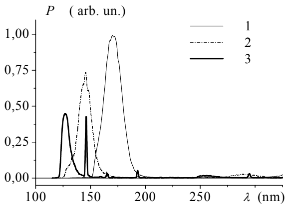
Fig. 3. Radiation spectra in Xe(1), Kr(2), Ar(3) at pressure of 1.2 atm at VDIAEB excitation
