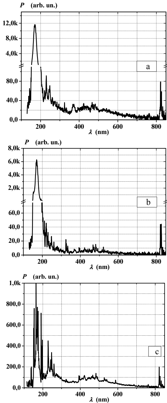
Fig. 4. A radiation spectrum of Xe in volume discharge at pressure of 1.2 atm (a), 0.3 atm (b); in contraction discharge, pressure – 0.3 atm (c)
