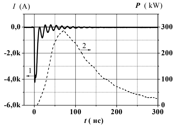
Fig. 5. Waveforms of current I(1) and VUV emission intensity P(2) ; Xe pressure – 1.2 atm
